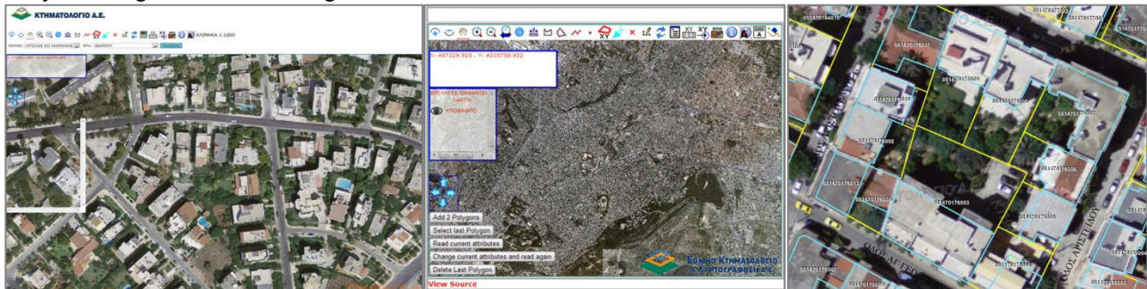
Fig.16-18: VLSO images data (GSD 20cm) of Chalandri via the Hellenic Cadastral Institution's web-GIS (fig.16), web-API (fig.17) and WMS-server (fig.18) [source: National Cadastre and Mapping Agency S.A. (EKXA S.A.)]
